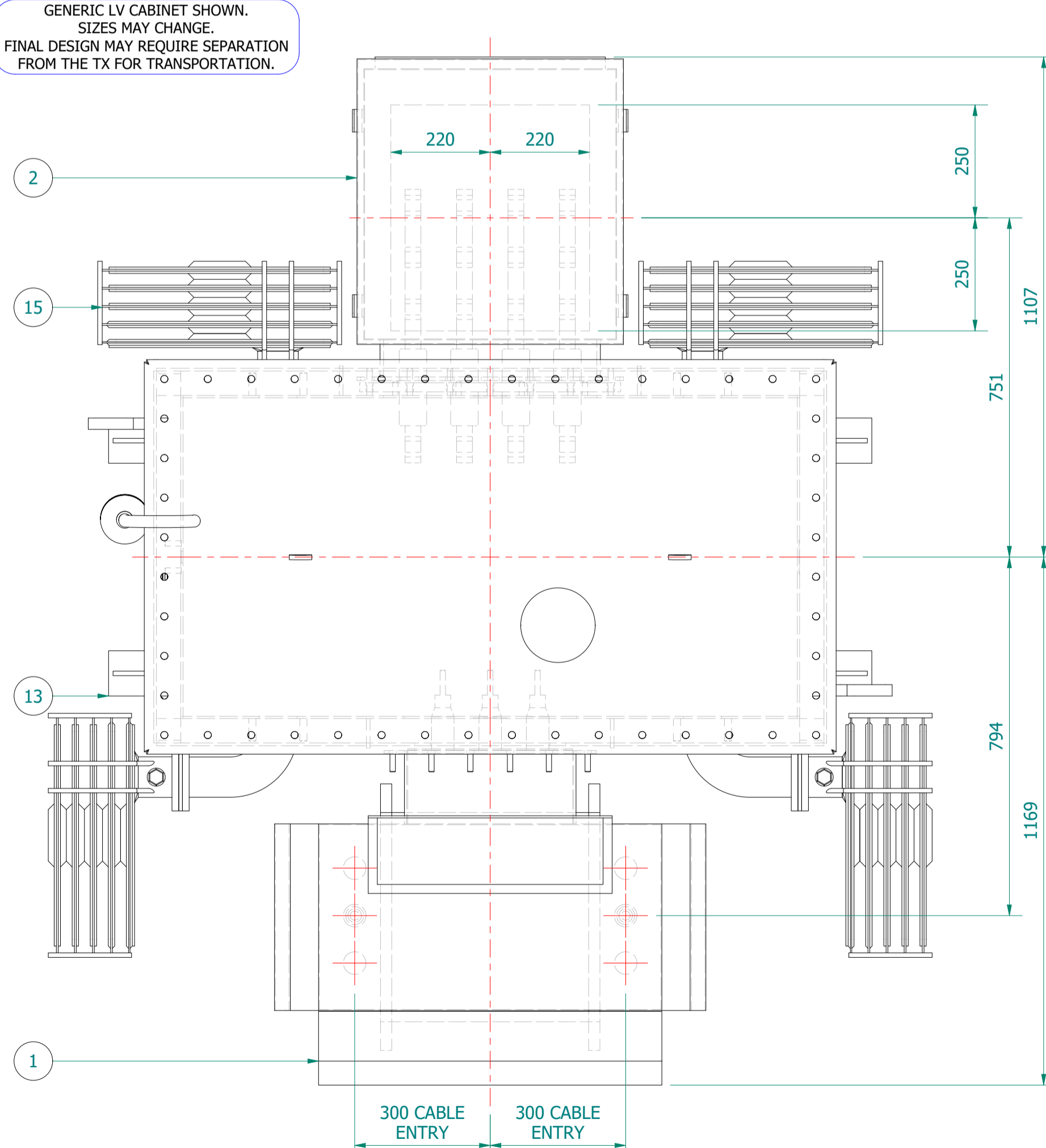
PLAN VIEW
