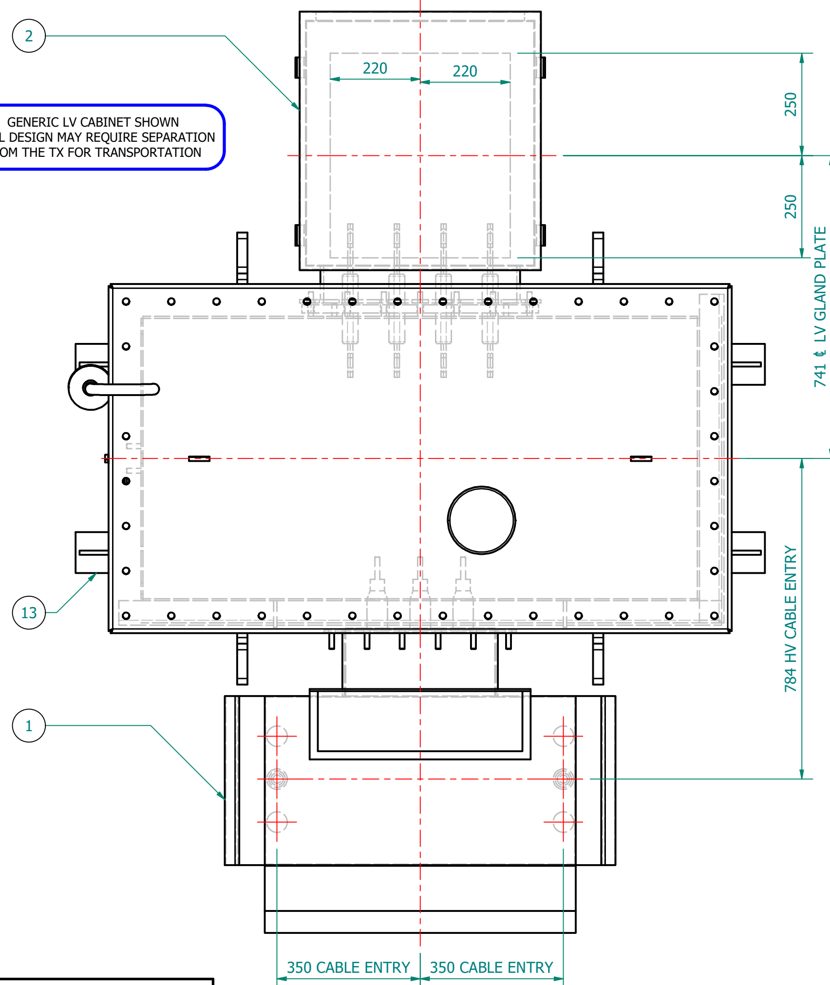
PLAN VIEW
