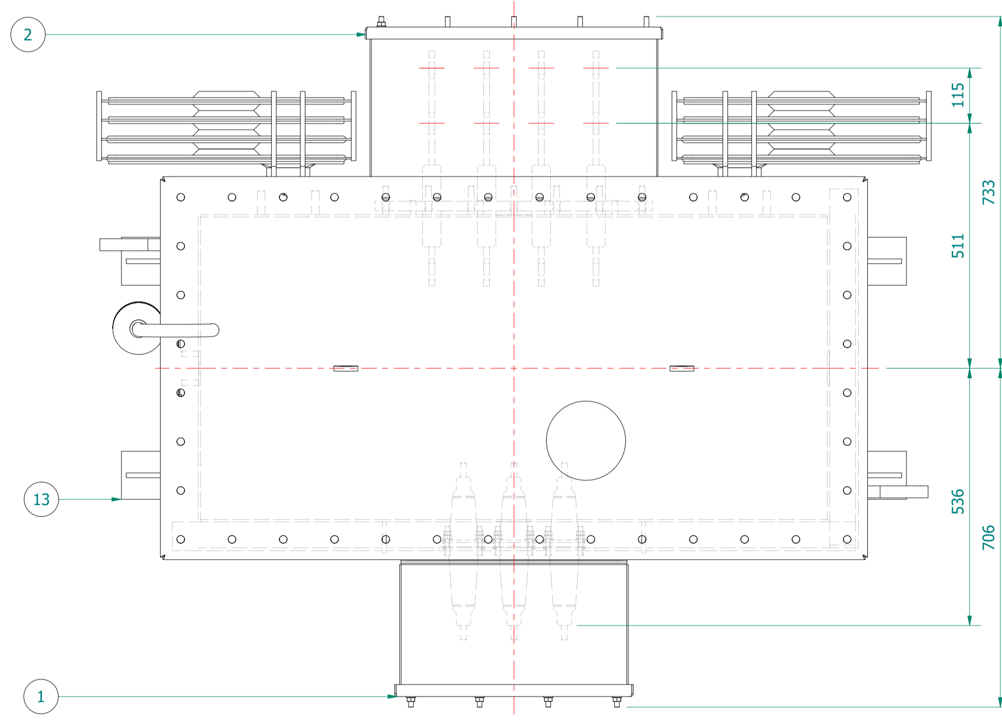
PLAN VIEW
