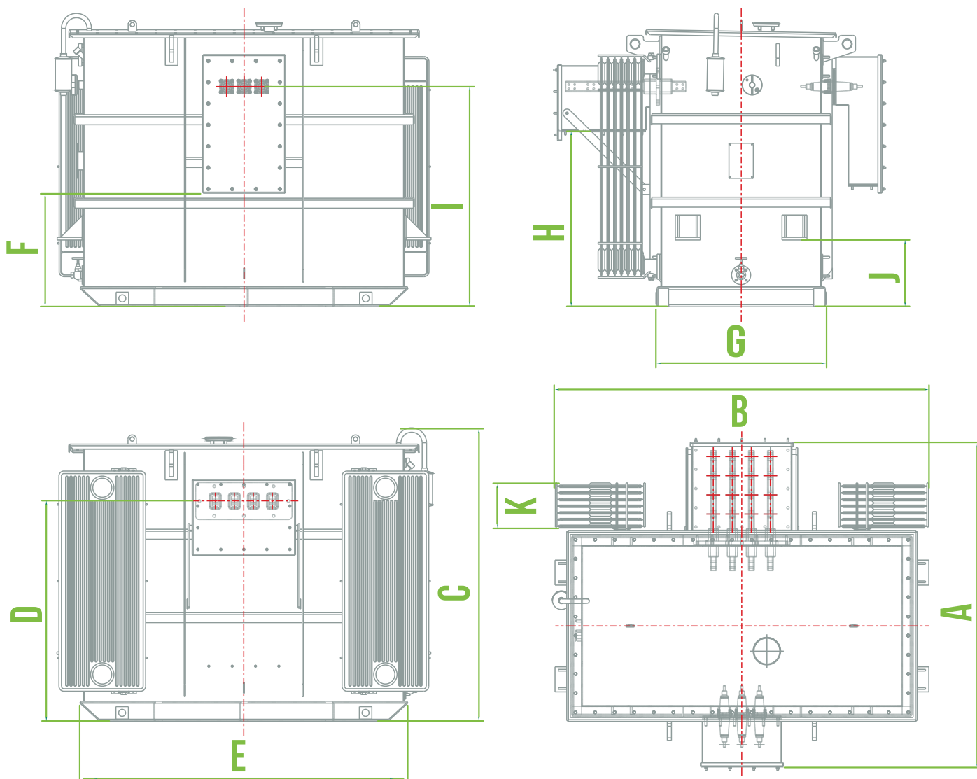
Representative general assembly shown for 2000kVA Wilson e4 transformer
